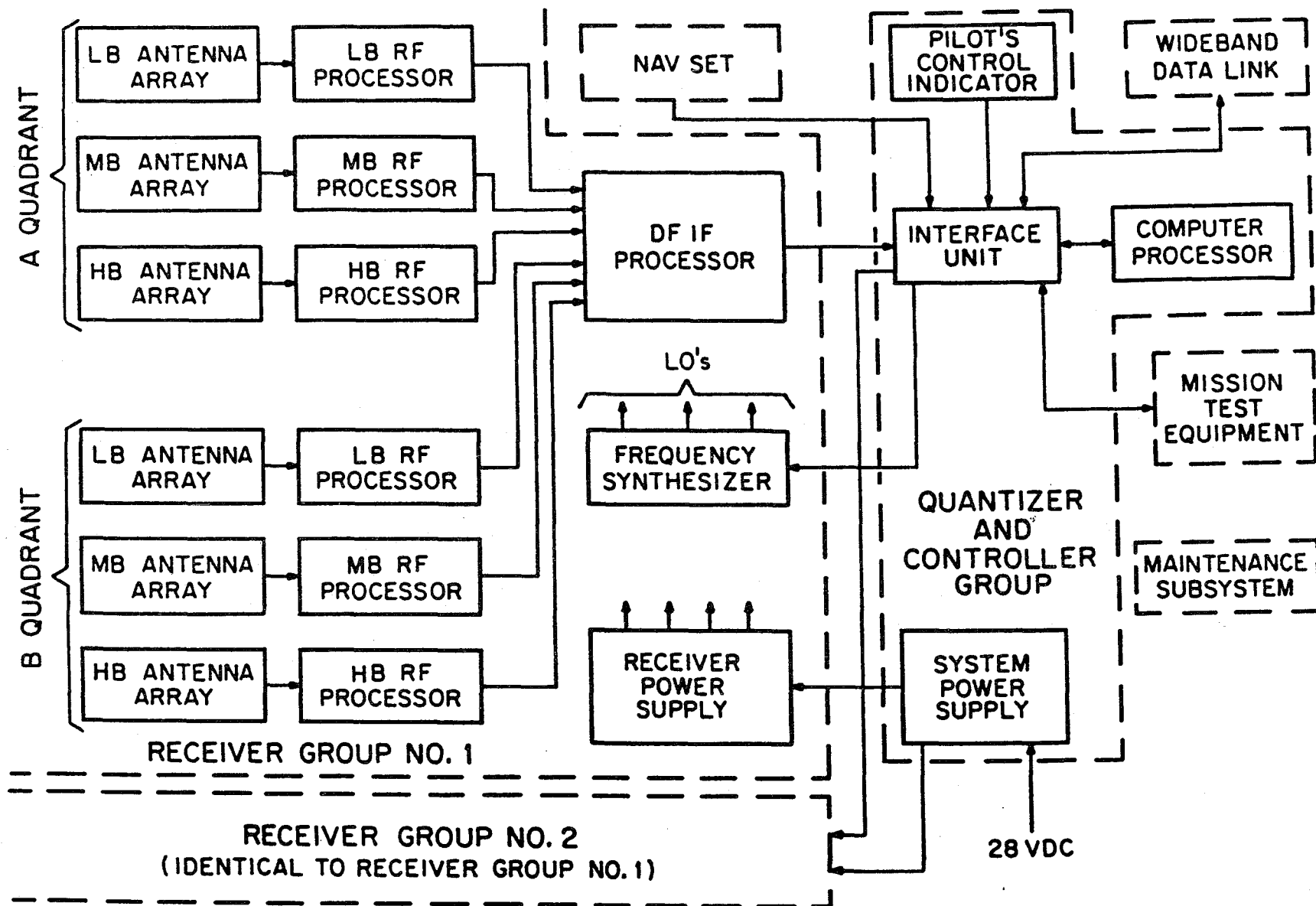
Figure 24. Block diagram of the Advanced QUICK LOOK airborne subsystem (ERADCOM, 1982).
