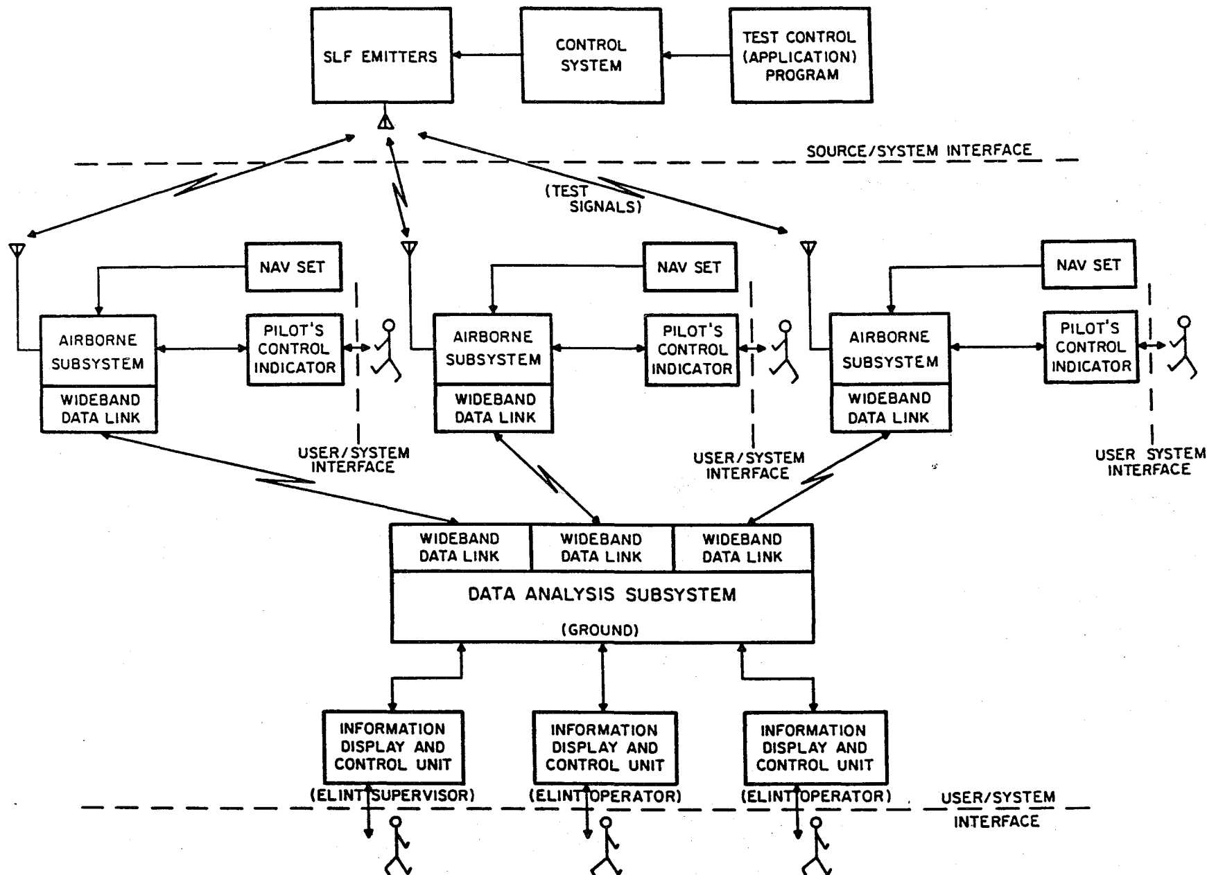
Figure 27. Simplified functional block diagram of the Advanced QUICK LOOK system showing source/system and user/system interfaces.
