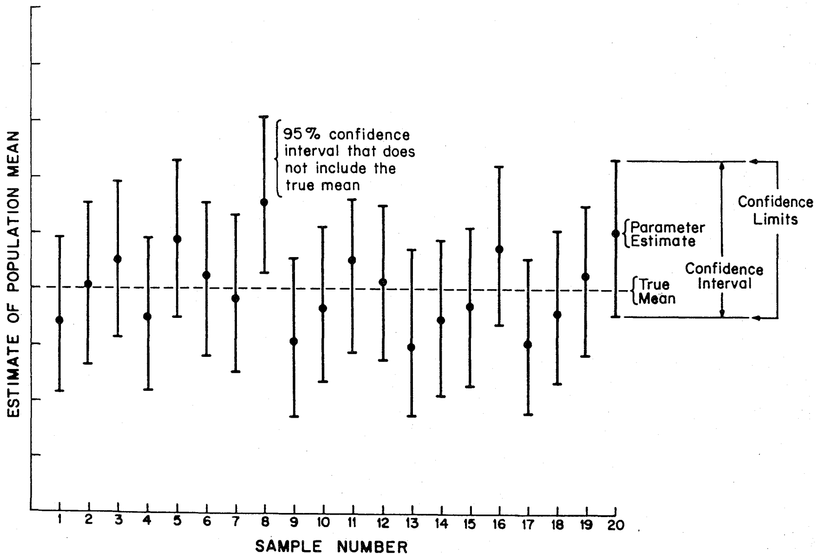
Figure 45. Illustration of 20 calculated confidence intervals (95% hypothetical) and the true mean for a parameter.
