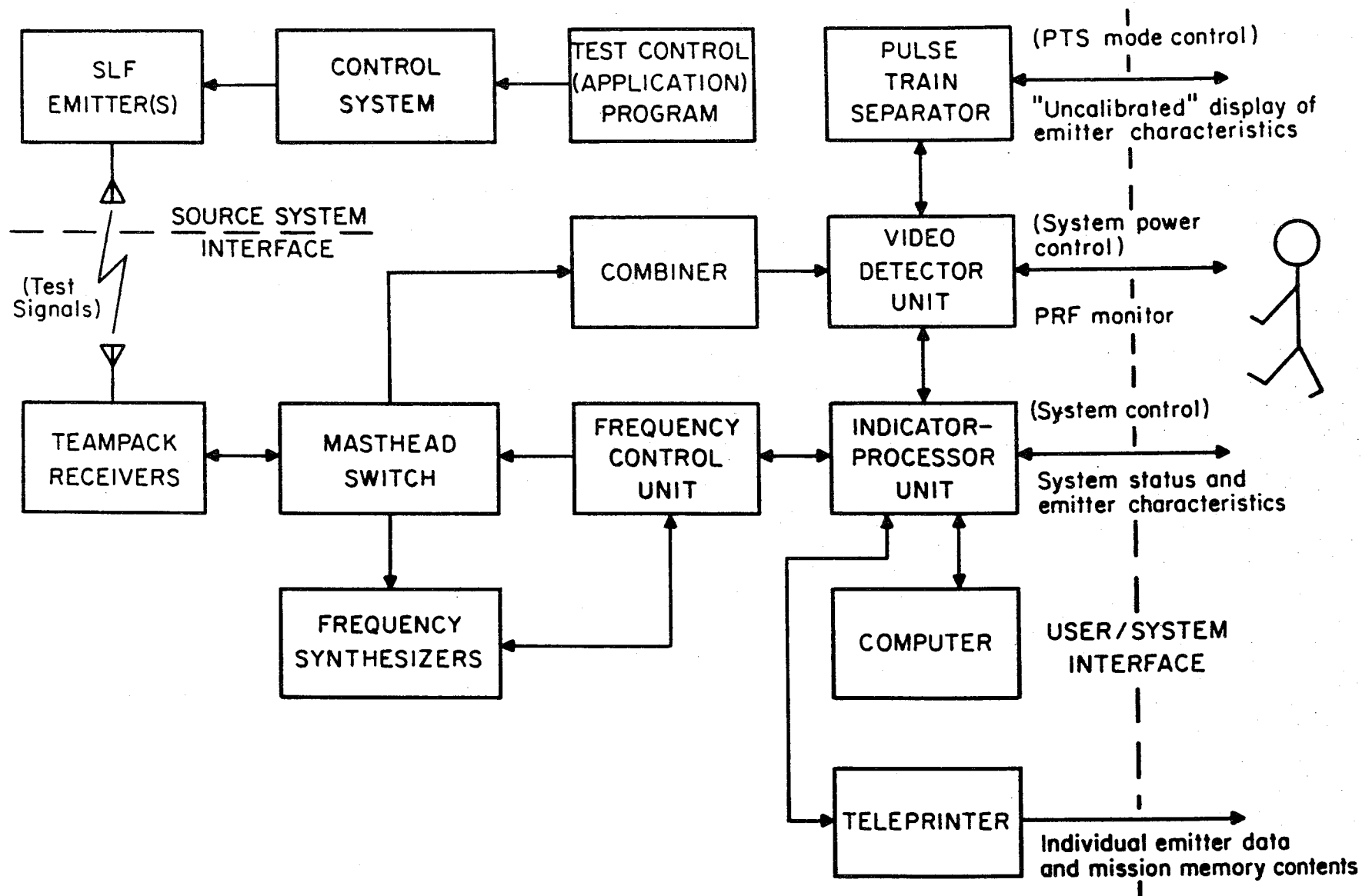
Figure 26. Simplified functional block diagram of the AN/MSQ-103 Receiver Set, Special Purpose (TEAMPACK Assembly) showing source/system and user/system interfaces and the (input)/output data.
