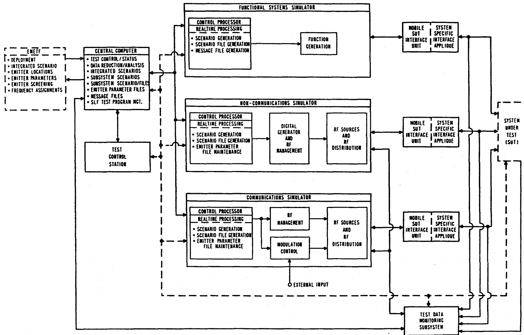
Figure 14. The functional SLF test concept and capability.
