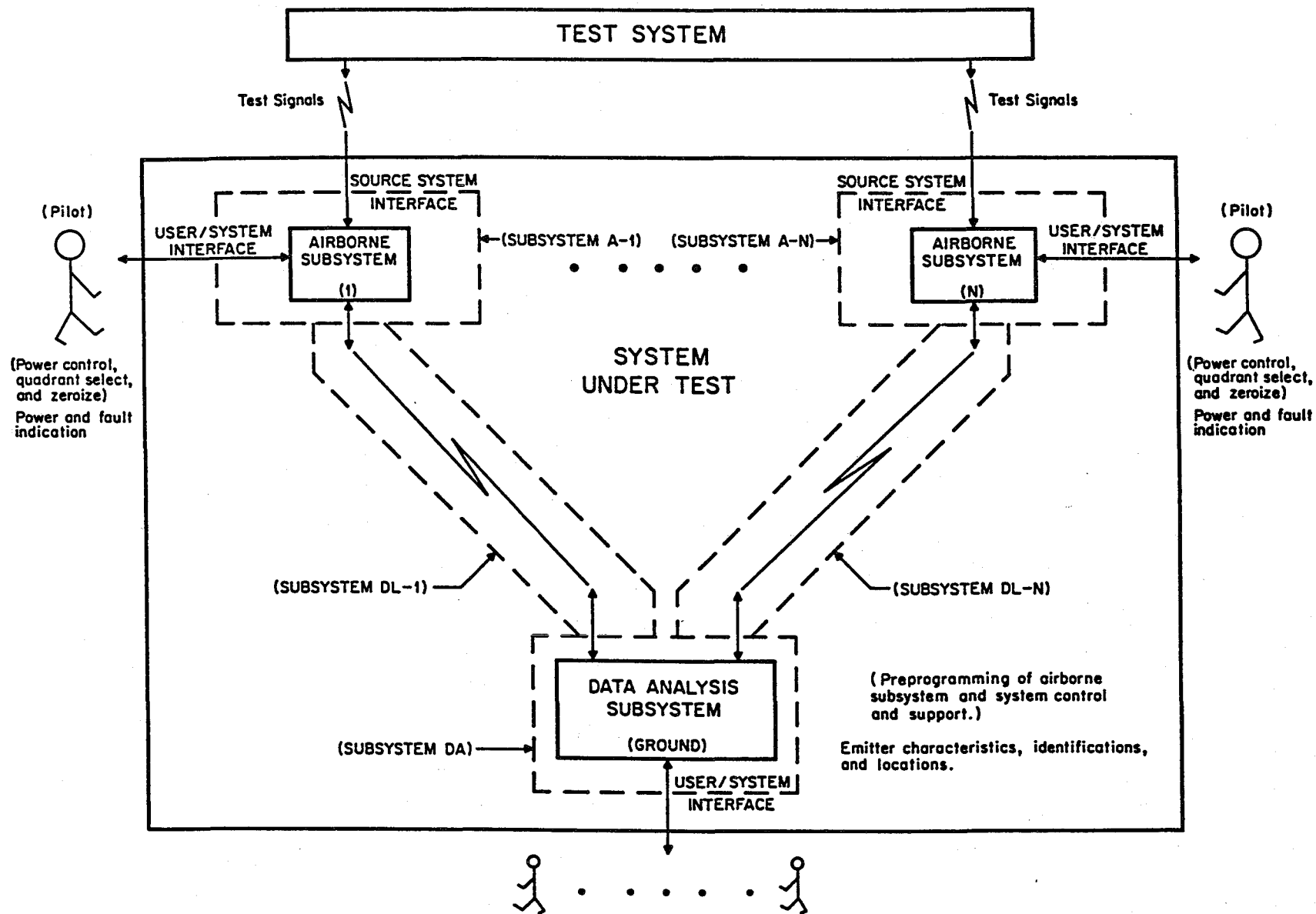
Figure 28. Further simplification to the functional block diagram of the Advanced QUICK LOOK System showing source/system and user/system interfaces and the (input)/output data.
