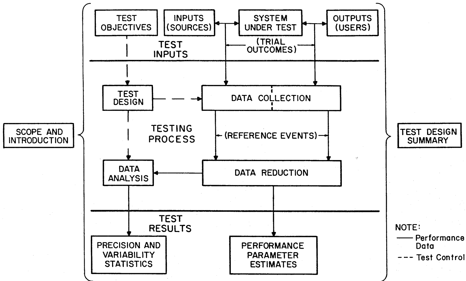
Figure 35. Generalized illustration of the system performance measurement process using system-independent measures of functional performance.
