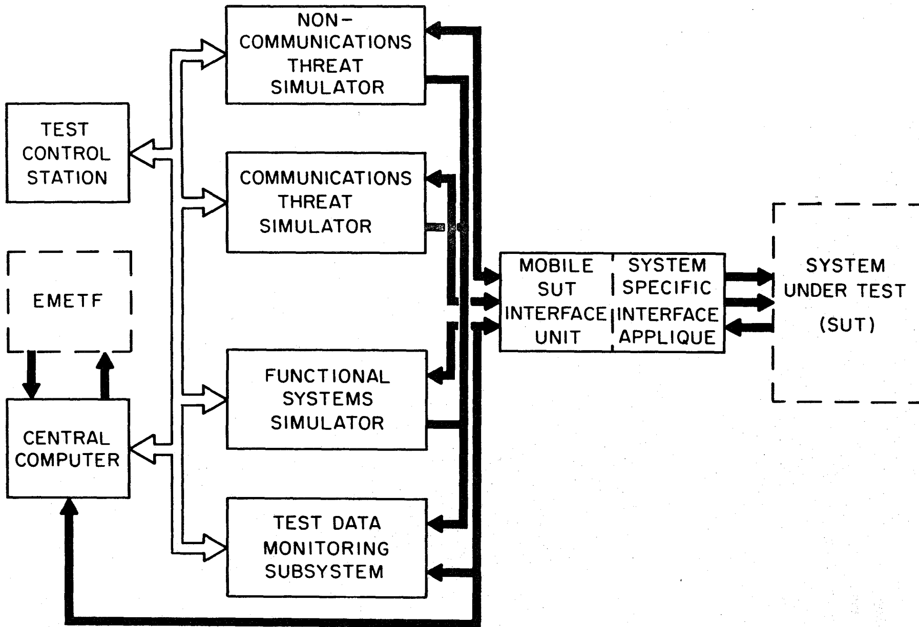
Figure 1. Simplified block diagram of the Stress Loading Facility (SLF) concept.
