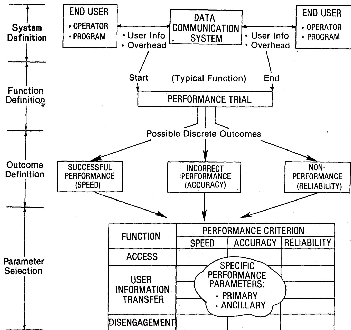
Figure B-1. The steps followed in ANSI X3.102-1983 to develop performance parameters for digital communication systems and services (ANSI, 1983).
