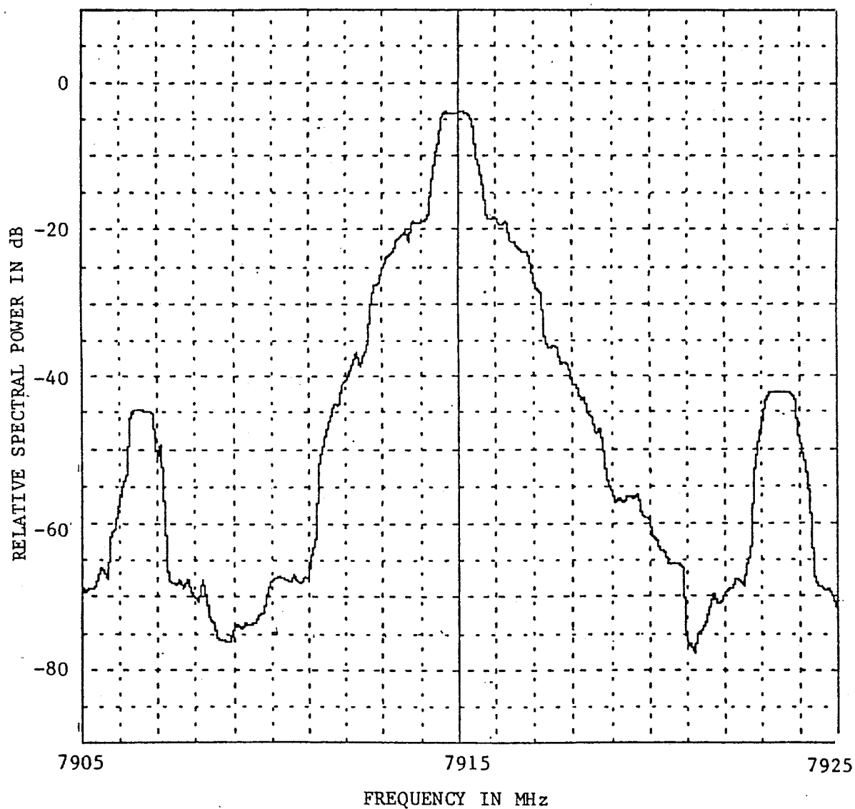
Figure A-29. Emission Spectrum of a General Electric TRS696C ( f_0 = 7915 MHz, Hard-lined).
