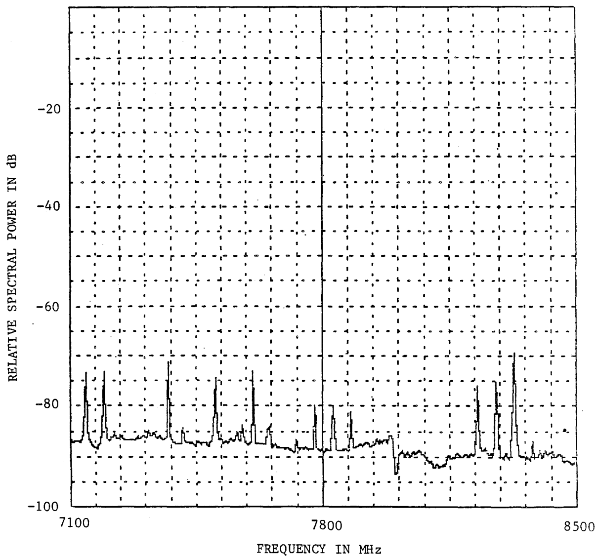
Figure A-6. Band Scan of the CG Station at Blyn Mountain- 7100-8500 MHz.
