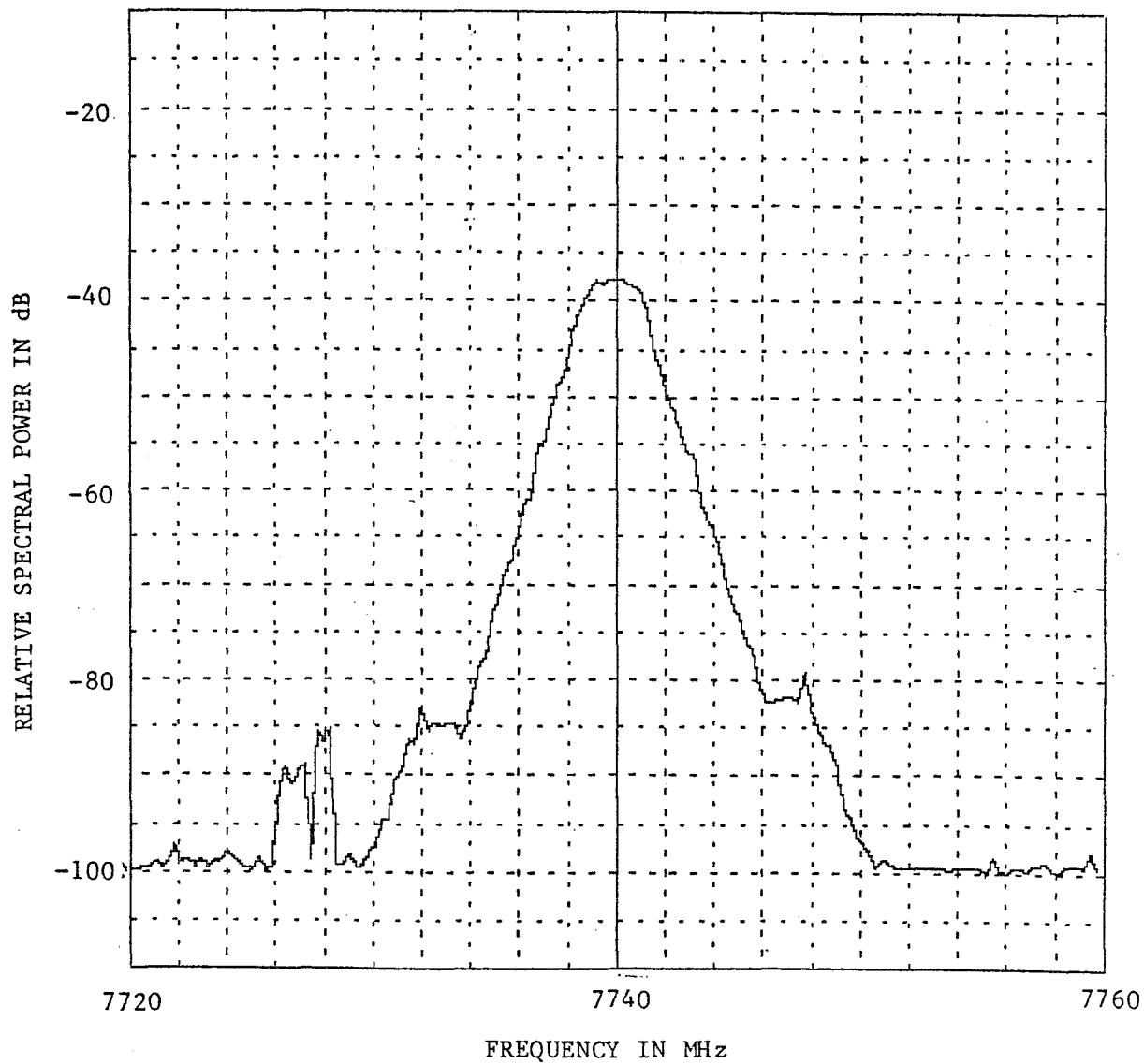
Figure A-49. Emission Spectrum of a COL MW508C ( f_o = 7740 MHz, Radiated, Normal Traffic).
