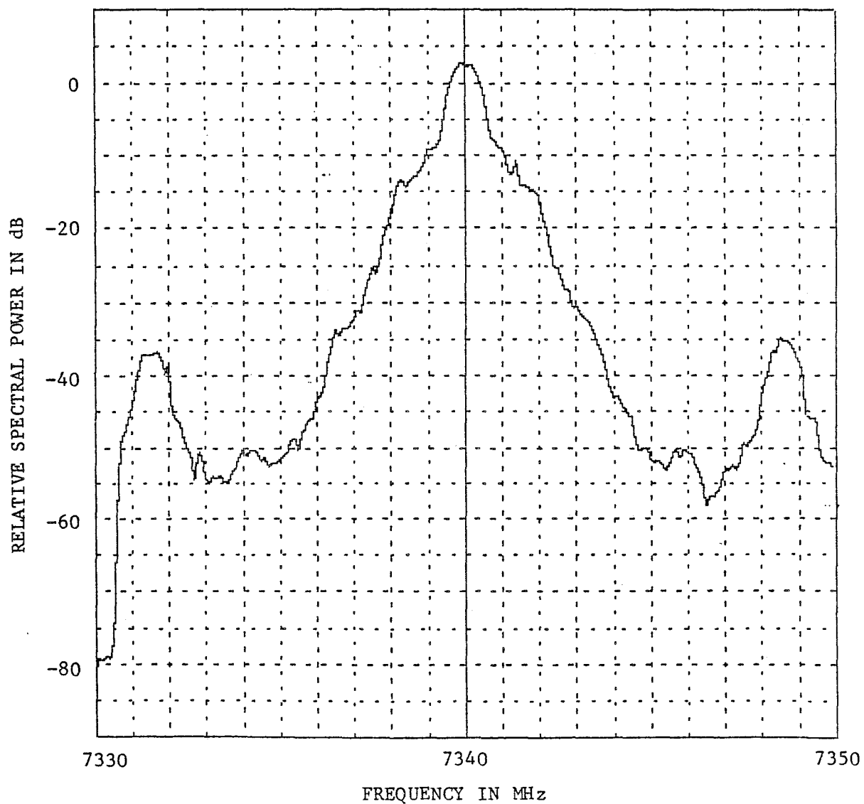
Figure A-38. Emission Spectrum of a GE TRS696C ( f_o = 7340 MHz, Hard-lined, Normal Traffic).
