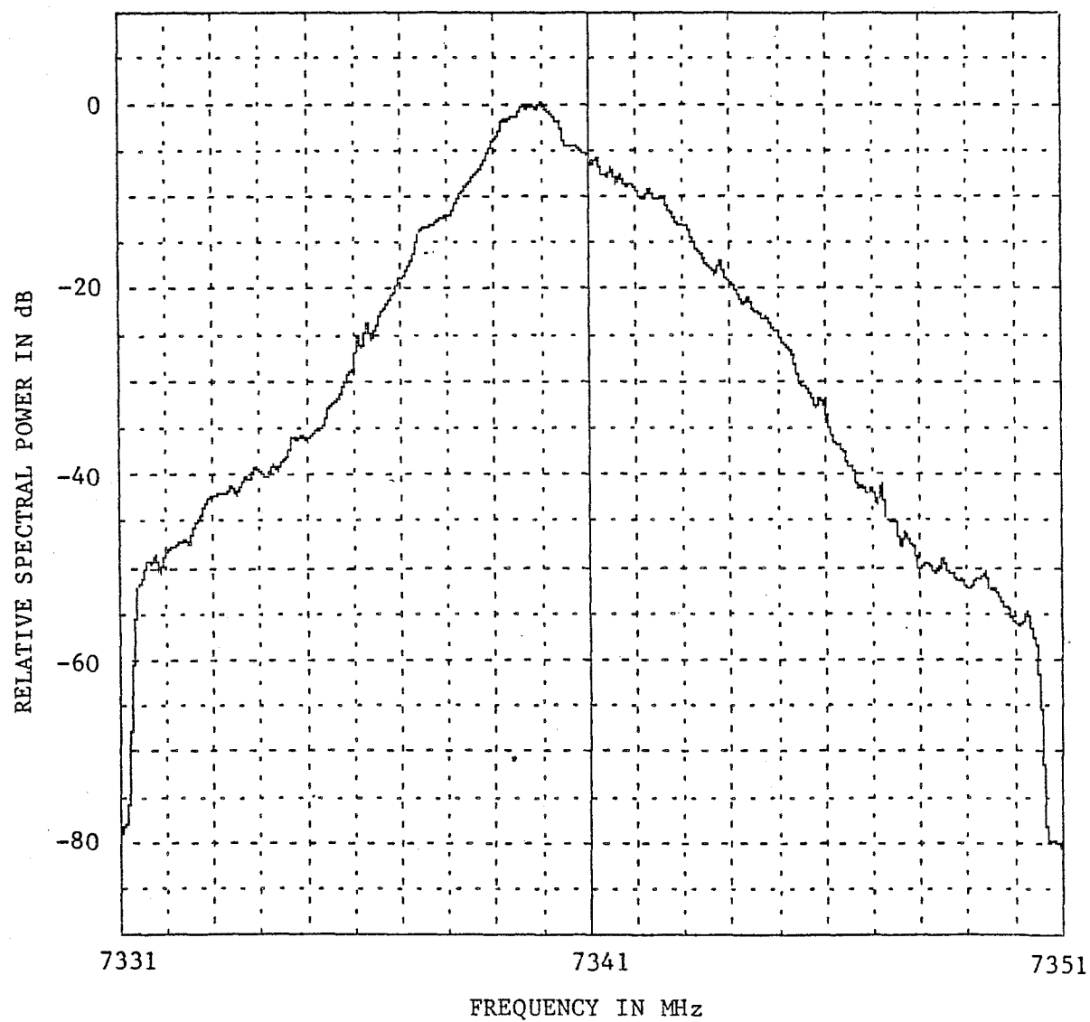
Figure A-40. Emission Spectrum of a GE TRS696C ( f_o = 7340 MHz, Hard-lined, Loaded Condition).
