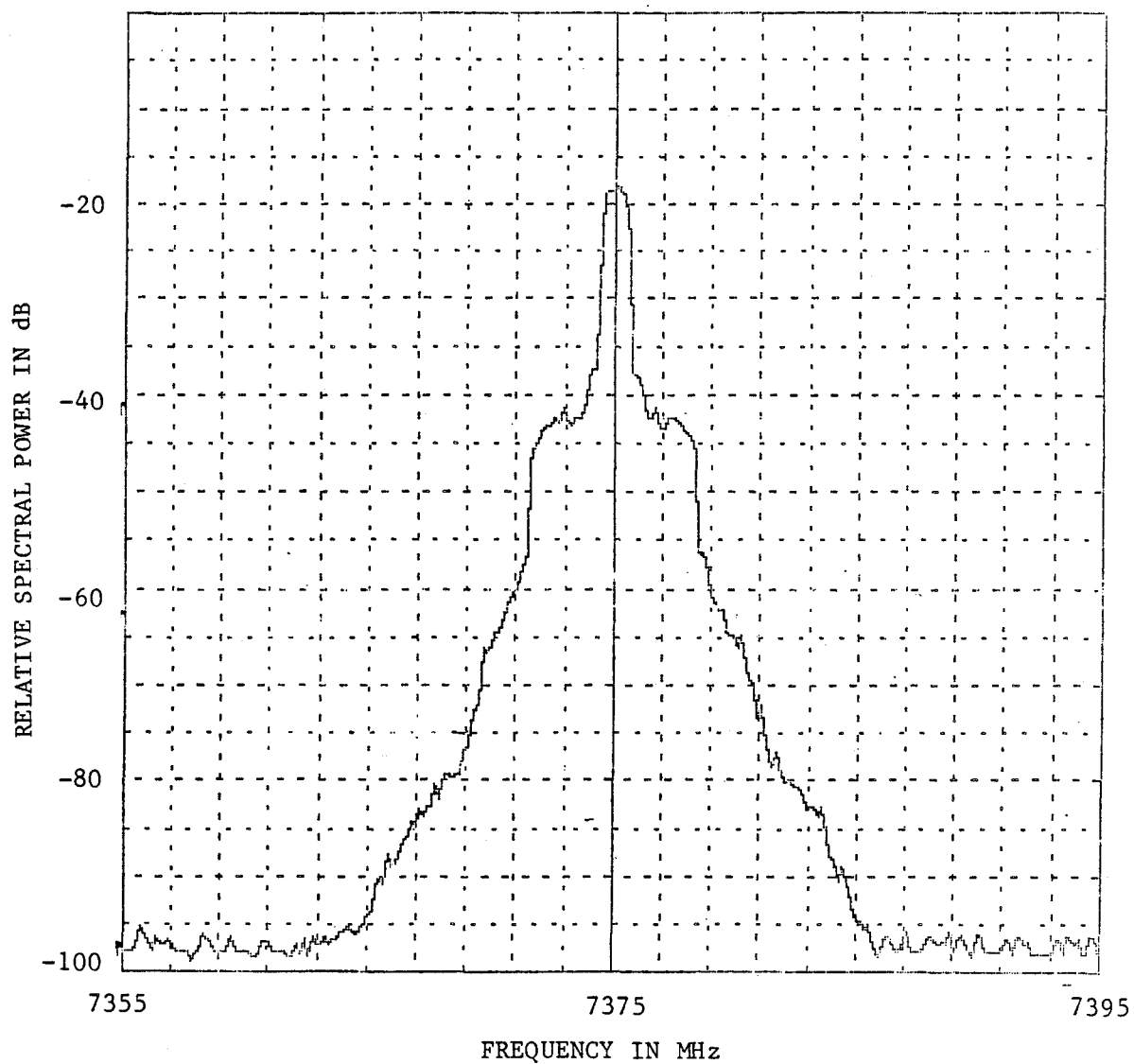
Figure A-2. Emission Spectrum of a Motorola MR300 Transmitter at Blyn Mountain ( f_0 = 7375 MHz).
