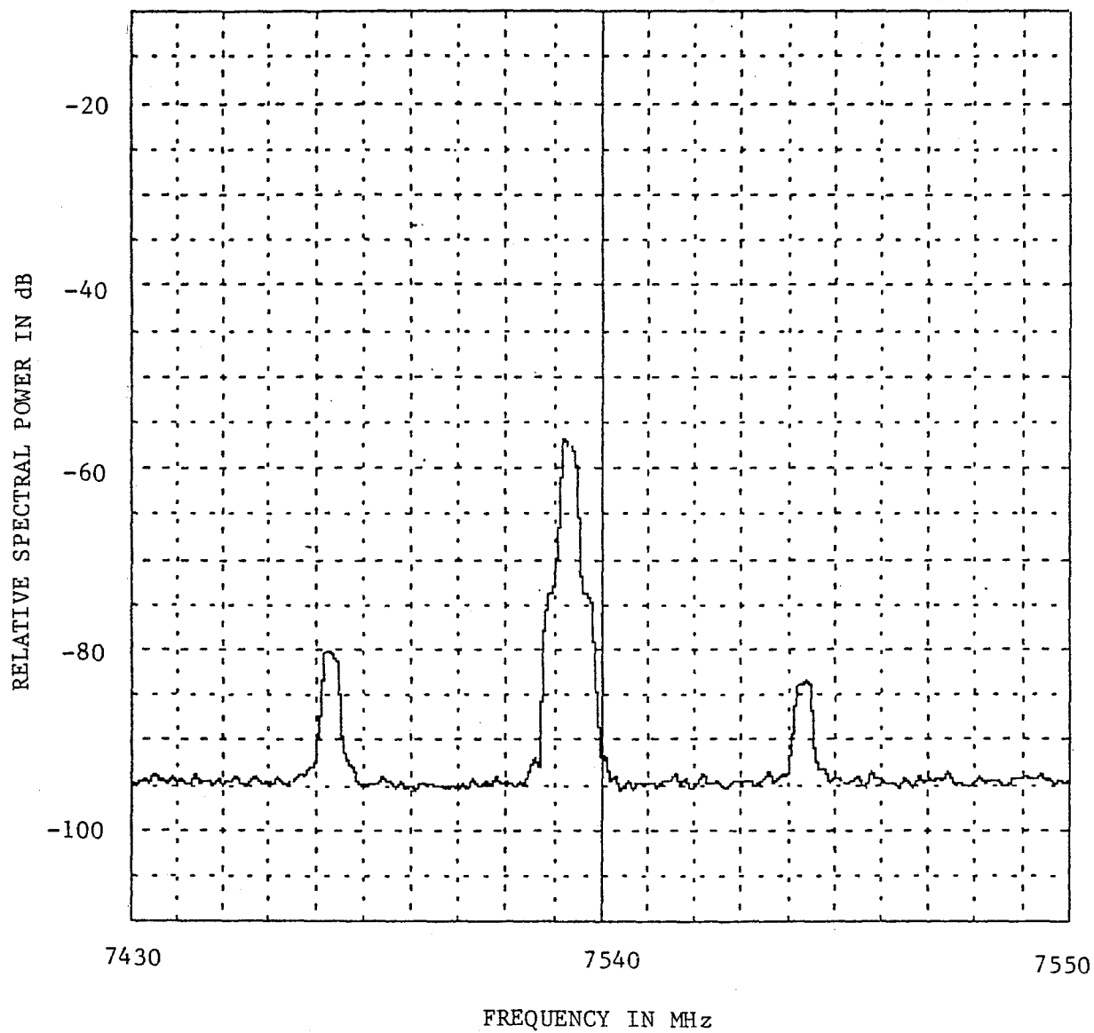
Figure A-59. Emission Spectrum of a Collins 552A-5 ( f_o = 7540 MHz, Radiated).
