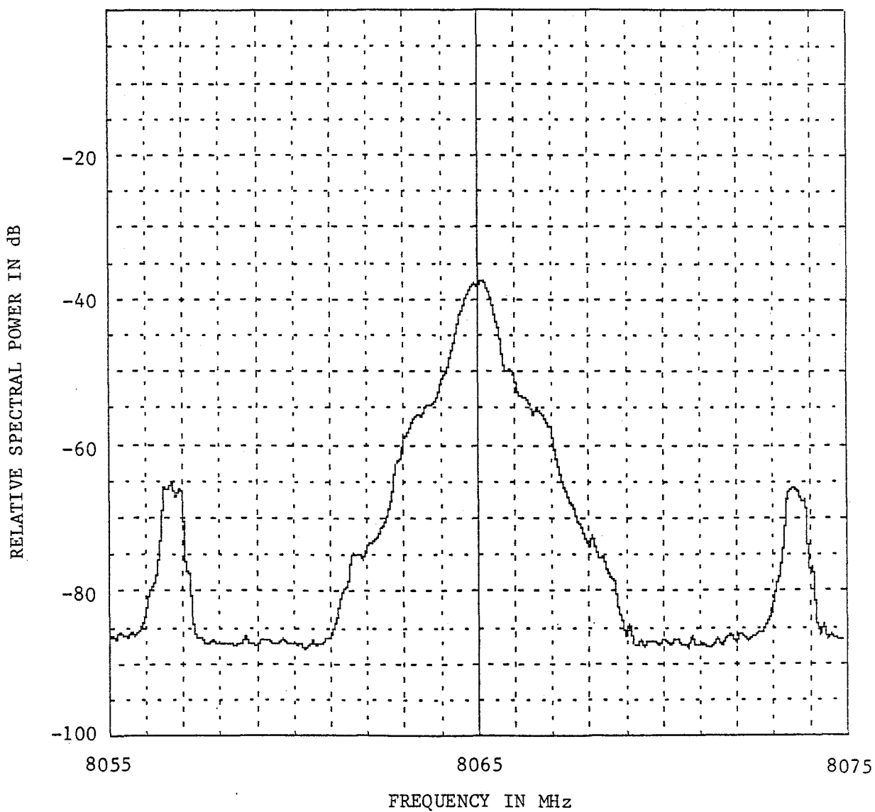
Figure A-25. Emission Spectrum of a General Electric TRS 696C ( f_o = 8065 MHz, Radiated).
