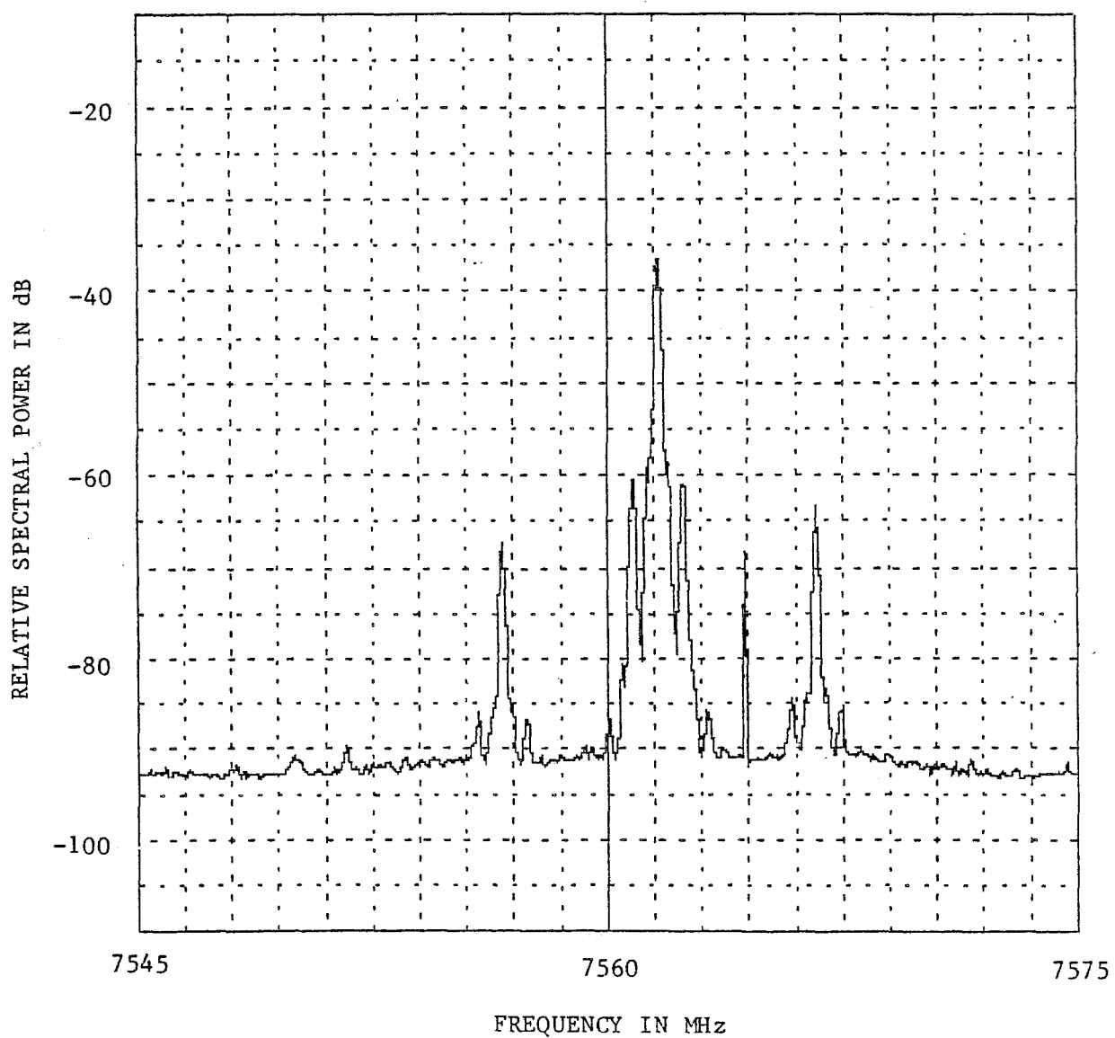
Figure A-66. Emission Spectrum of a Collins 552A-5 ( f_o = 7560 MHz, Radiated).
