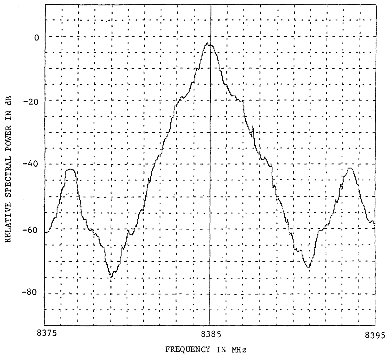
Figure A-32. Emission Spectrum of a General Electric TRS696C ( f_0 = 8385 MHz, Hard-lined).
