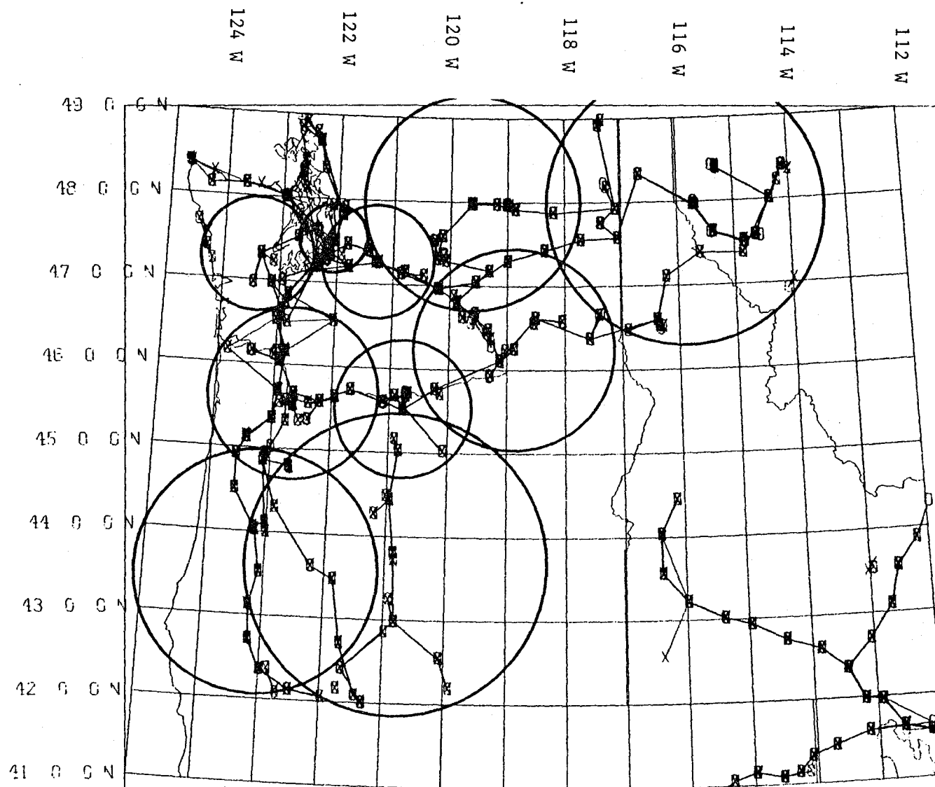
Figure B-4. Geographic Distribution of Frequency Assignments in the Pacific Northwest in the 7125-8400 MHz Band.
