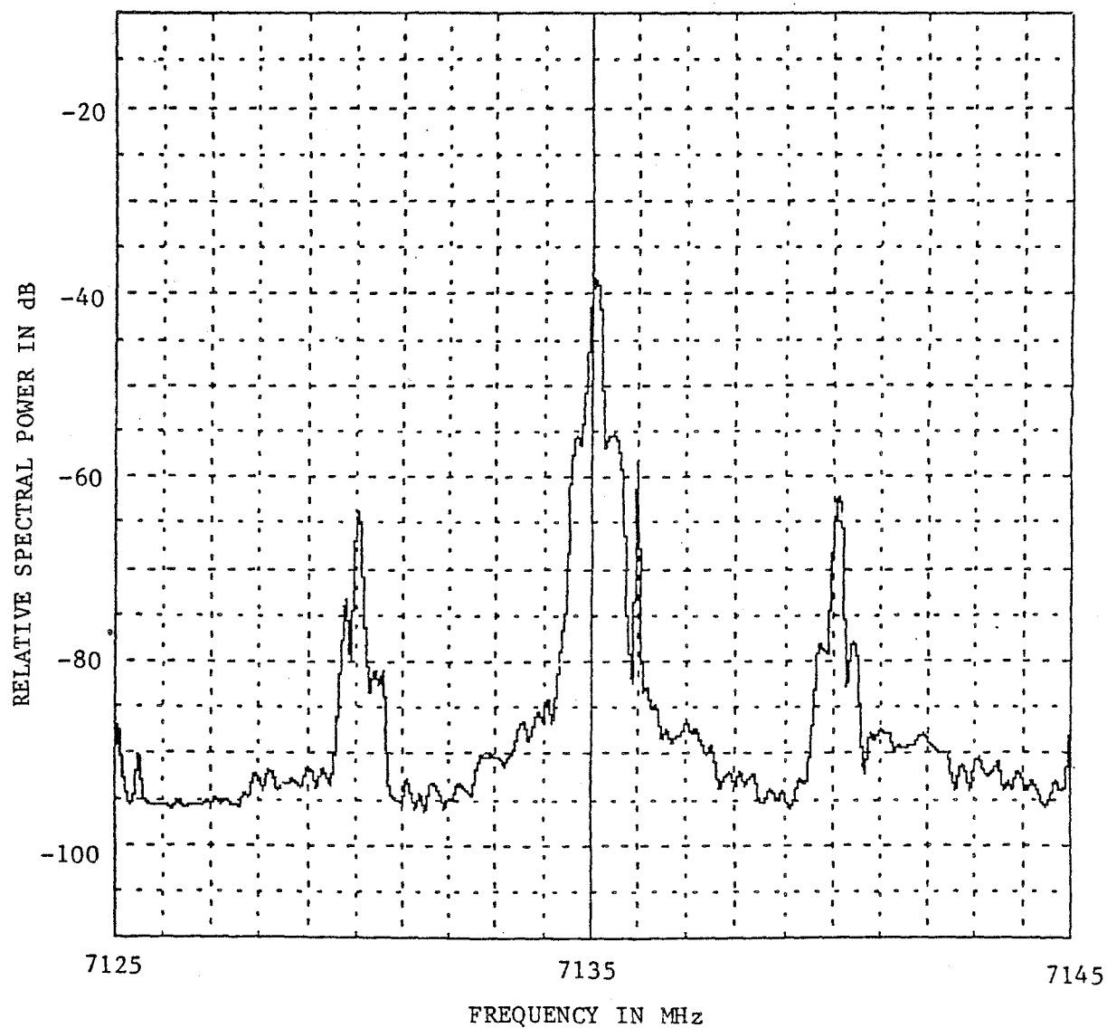
Figure A-54. Emission Spectrum of a Collins 552 A-5 ( f_o = 7135 MHz, Radiated).
