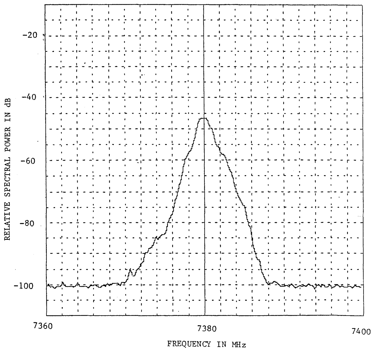
Figure A-47. Emission Spectrum of a COL MW508C ( f_o = 7380 MHz, Radiated, Loaded Condition).
