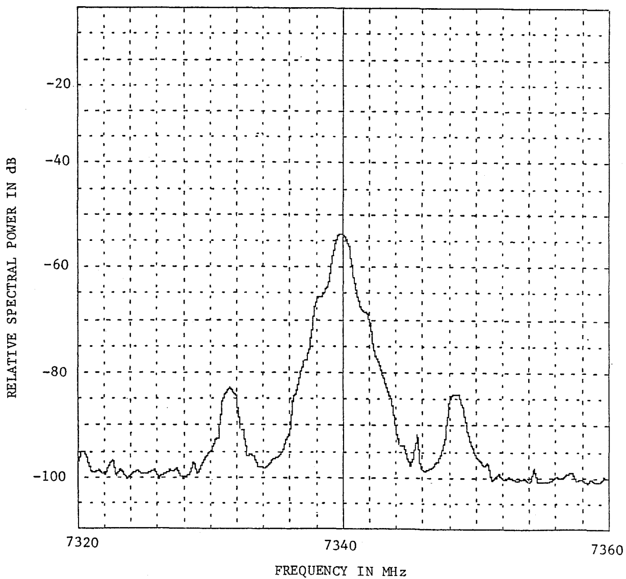
Figure A-37. Emission Spectrum of a GE TRS696C ( f_o = 7340 MHz, Radiated, Normal Traffic).
