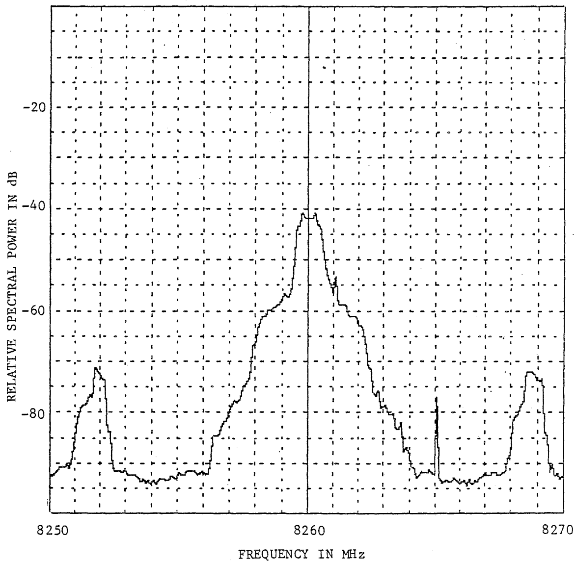
Figure A-24. Emission Spectrum of a General Electric TRS 696C ( f_o = 8260 MHz, Radiated).
