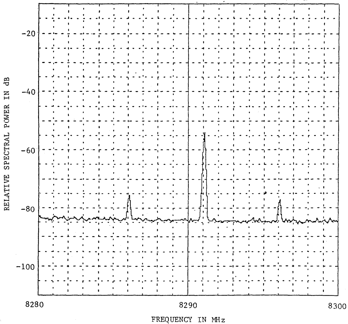
Figure A-62. Emission Spectrum of Collins 552A-5 ( f_o = 8290 MHz, Radiated).
