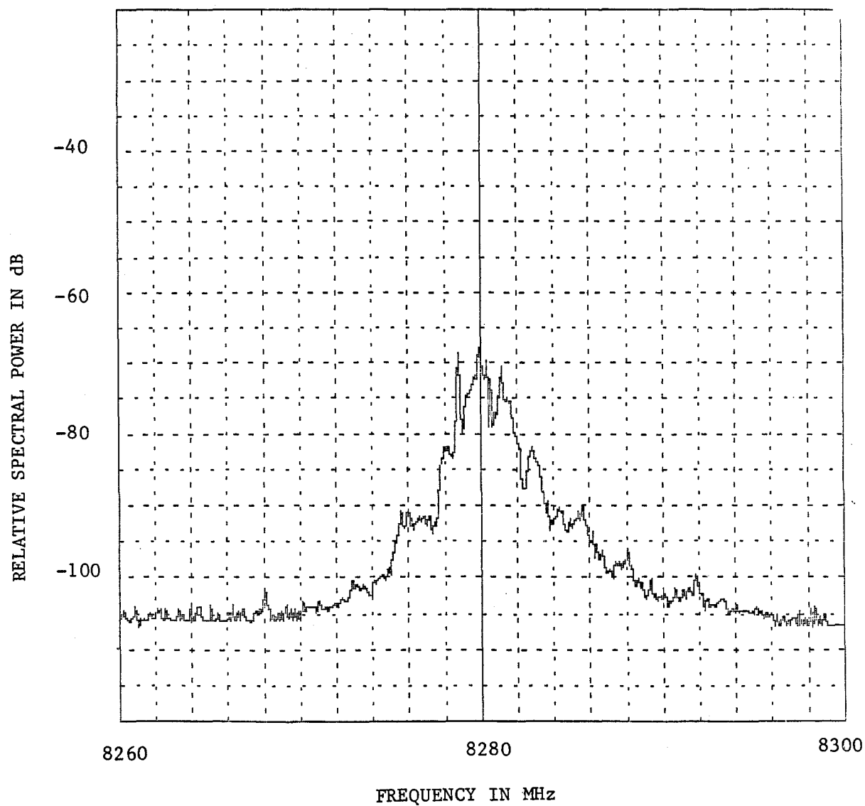
Figure A-11. Emission Spectrum of a Farinon Electric FV8F, ( f_o = 8280 MHz, Radiated).
