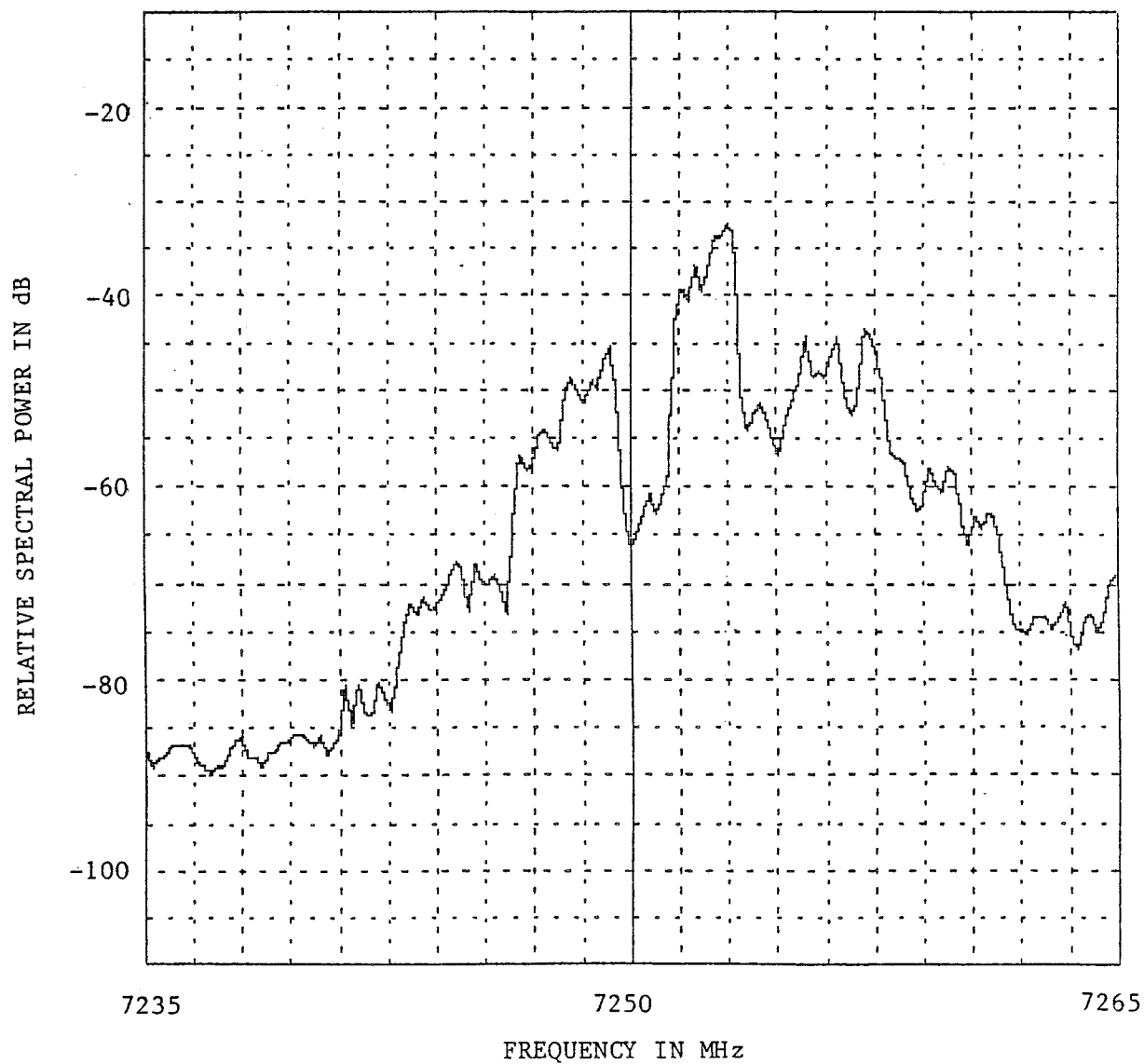
Figure A-70. Emission Spectrum of a Collins 552A-5 ( f_o = 7250 MHz, Radiated).
