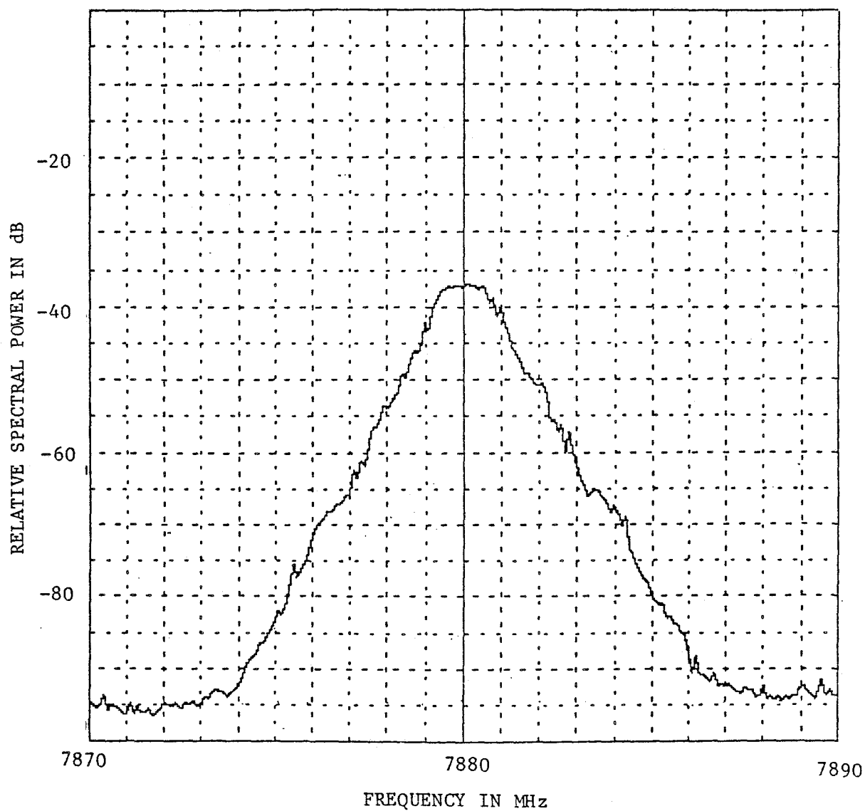
Figure A-28. Emission Spectrum of a Collins MW508D ( f_o = 7880 MHz, Radiated)
