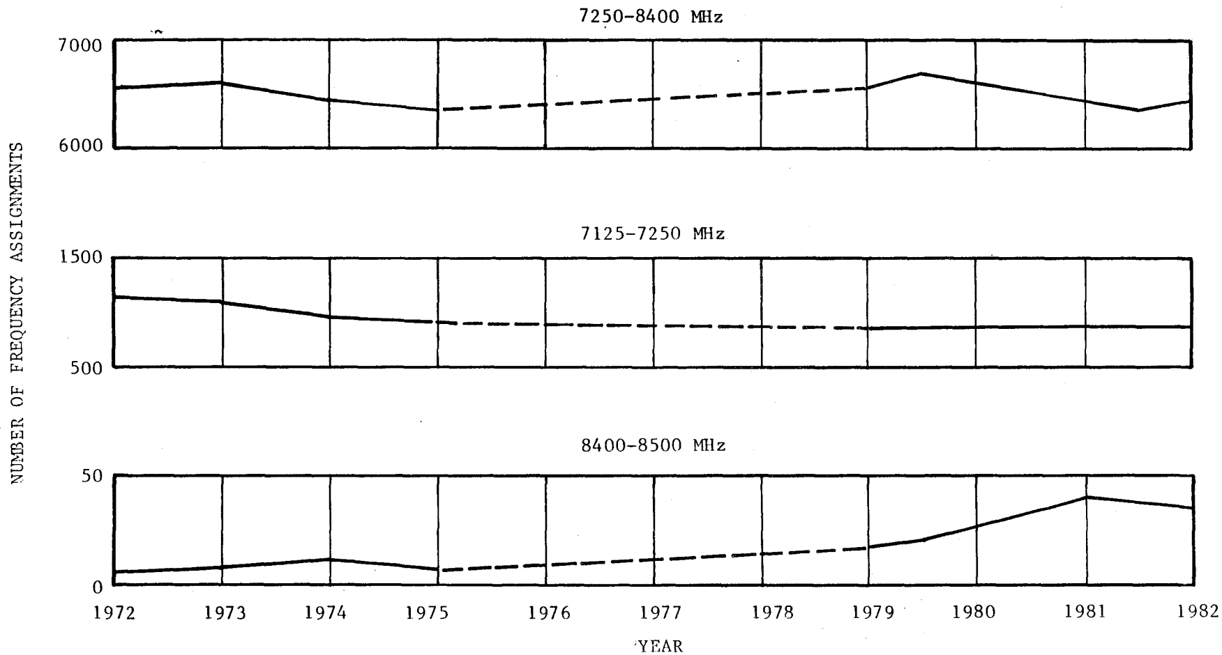
Figure 8. Number of Frequency Assignments in the 7125-8500 MHz Band Per Year
