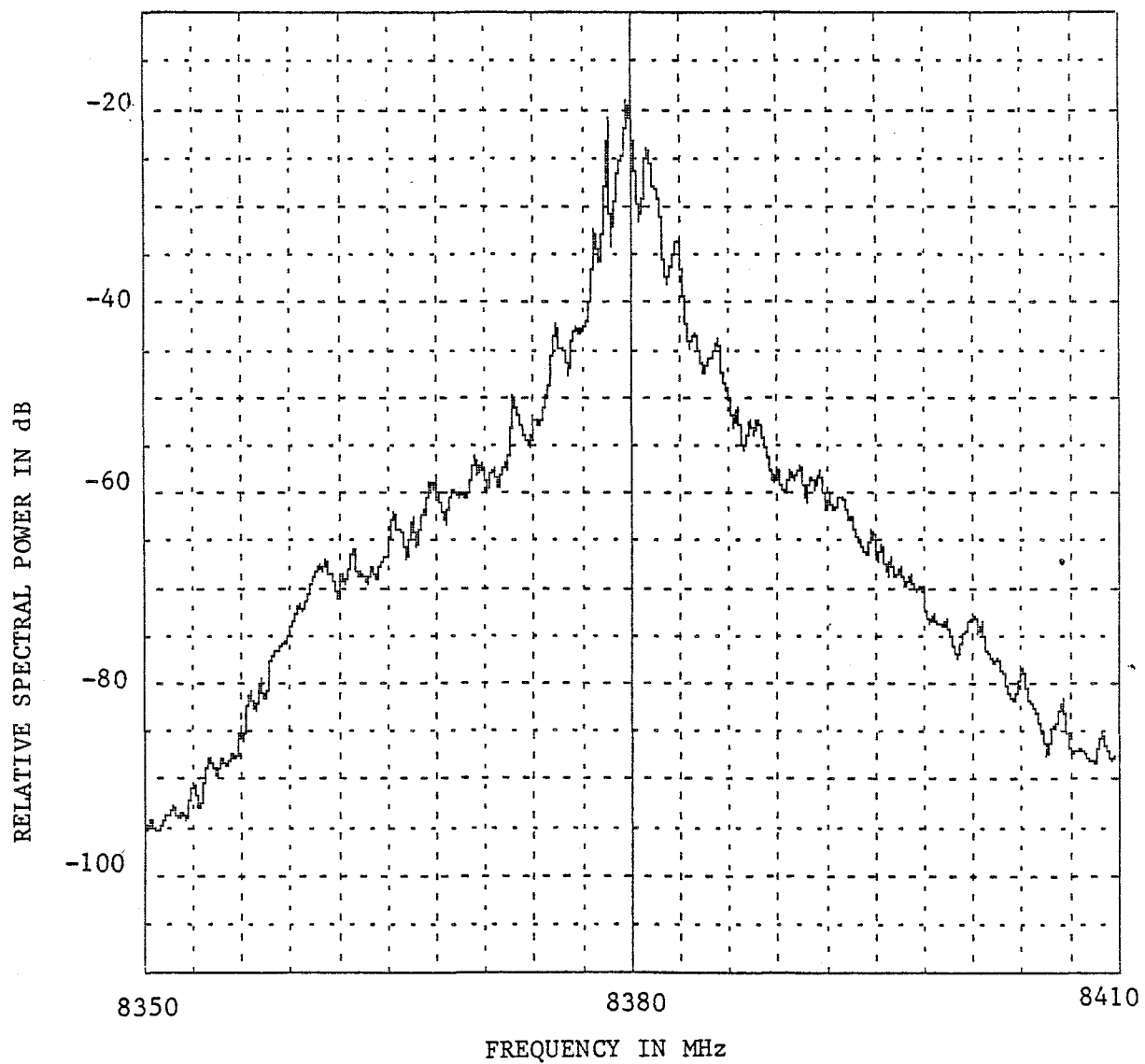
Figure A-20, Emission Spectrum of a Farinon Electric FV8F ( f_o = 8380 MHz, Hard-lined).
