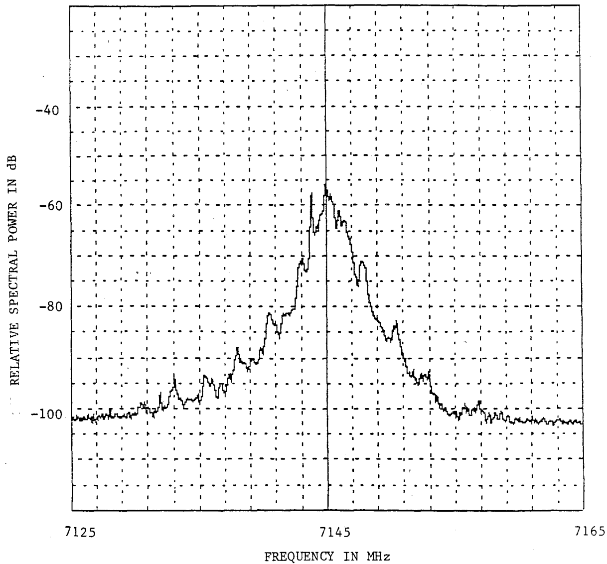
Figure A-7. Emission Spectrum of a Farinon Electric FV8F ( f_0 = 7145 MHz, Radiated).
