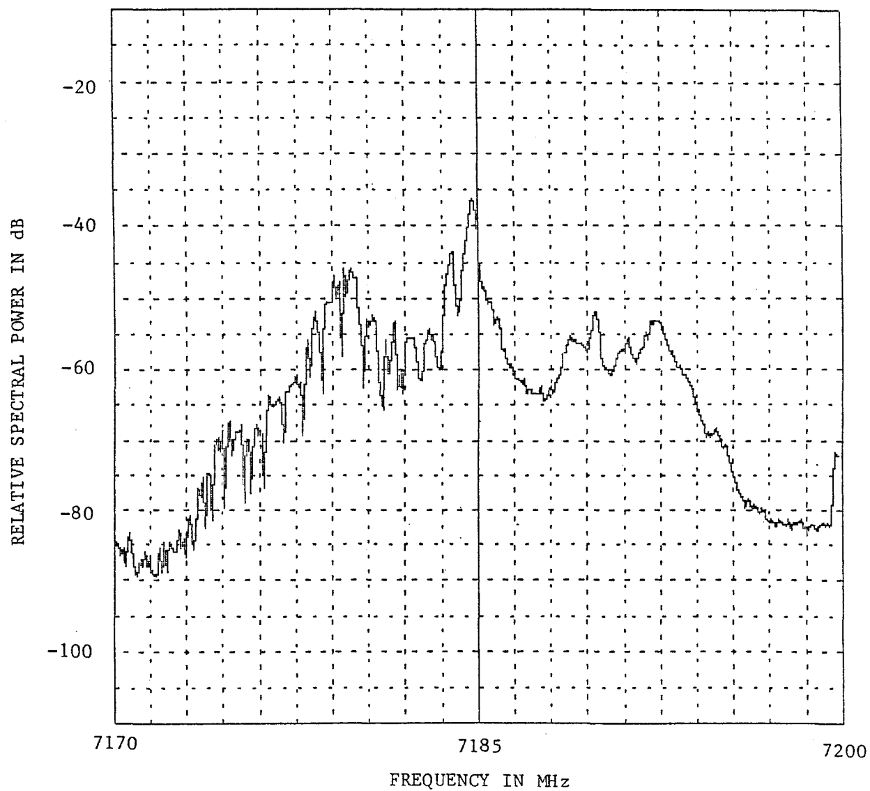
Figure A-69. Emission Spectrum of a Collins 552A-5 ( f_o = 7185 MHz, radiated).
