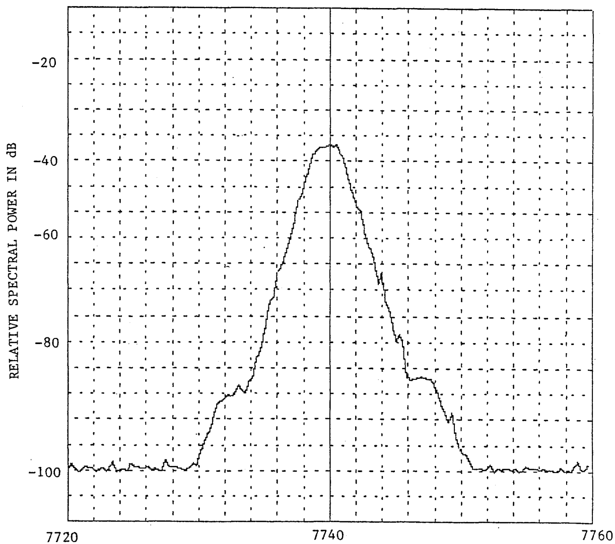
Figure A-51. Emission Spectrum of a COL MW508C ( f_o = 7740 MHz, Radiated, Loaded Condition).
