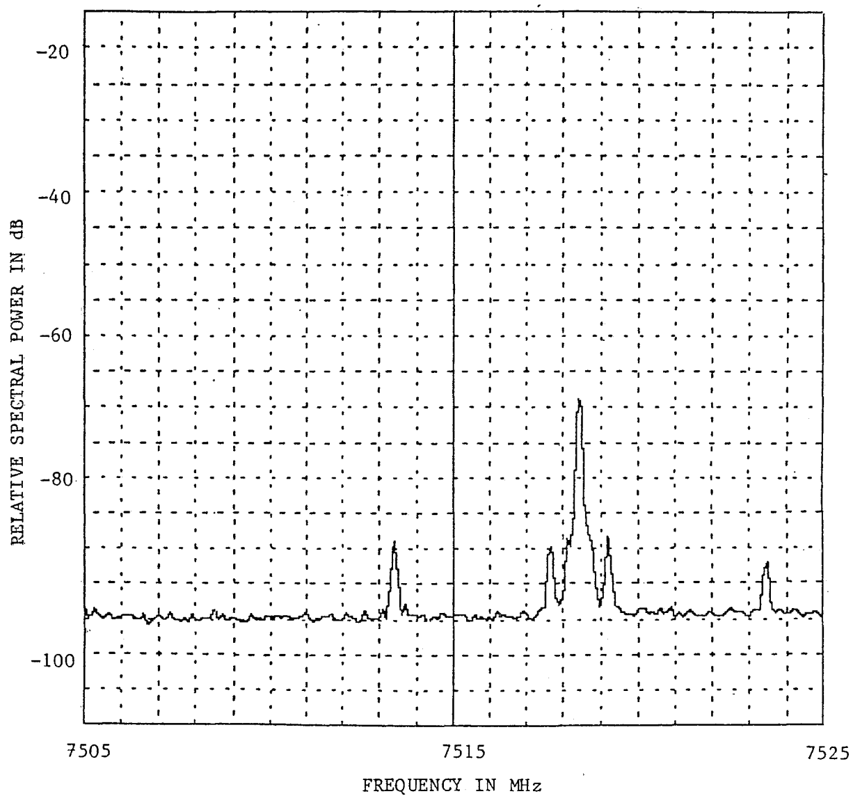
Figure A-57. Emission Spectrum of a Collins 552A-5 ( f_o = 7515 MHz, Radiated).
