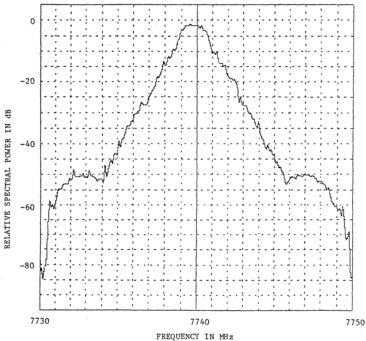
Figure A-50. Emission Spectrum of a COL MW508C ( f_o = 7740 MHz, Hard-lined, Normal Traffic).
