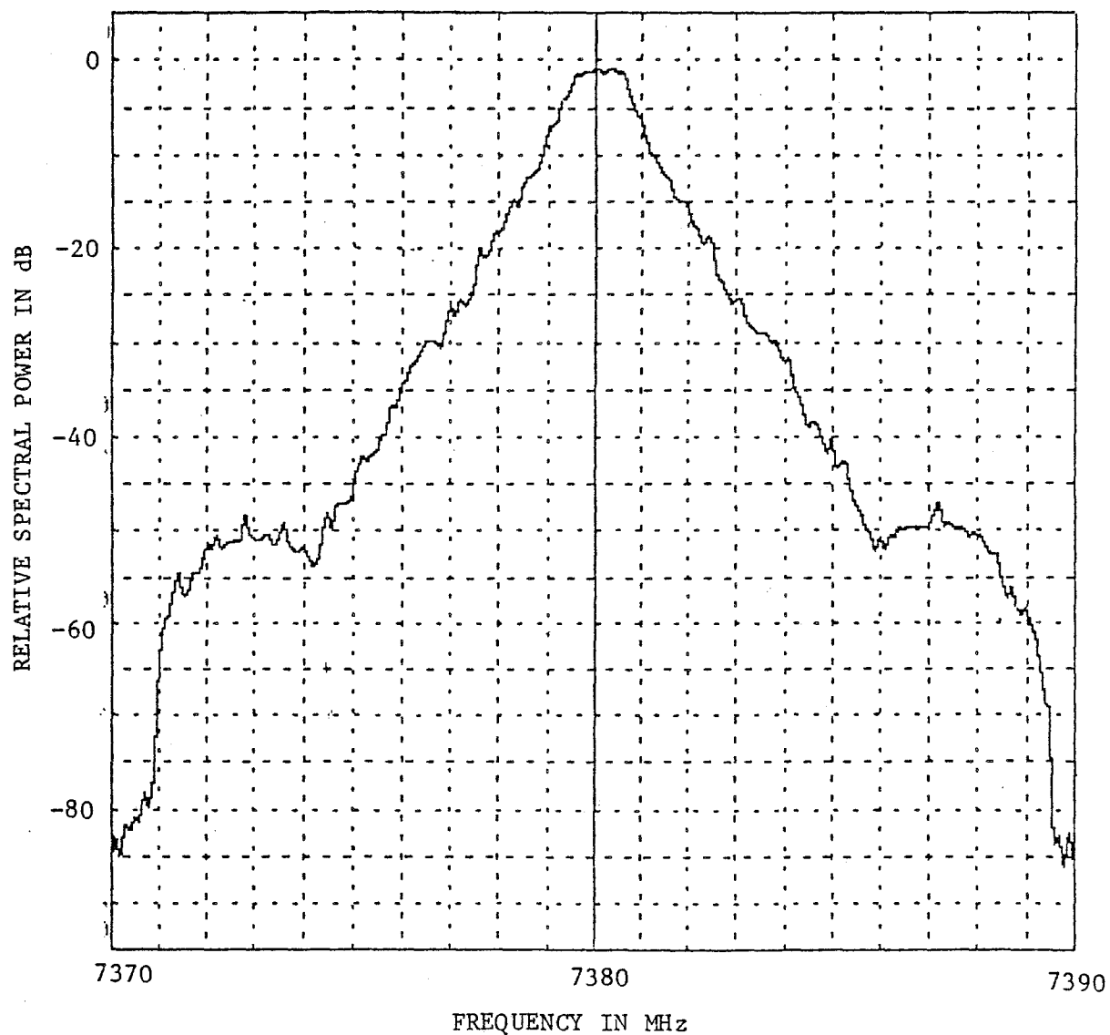
Figure A-46. Emission Spectrum of a COL MW508C ( f_o = 7380 MHz, Hard-lined, Normal Traffic).
