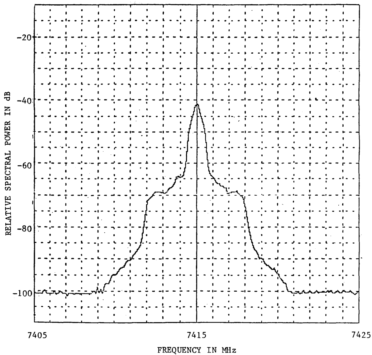
Figure A-5. Emission Spectrum of a Motorola MR300 Transmitter at Bangor, Washington ( f_o = 7415 MHz).
