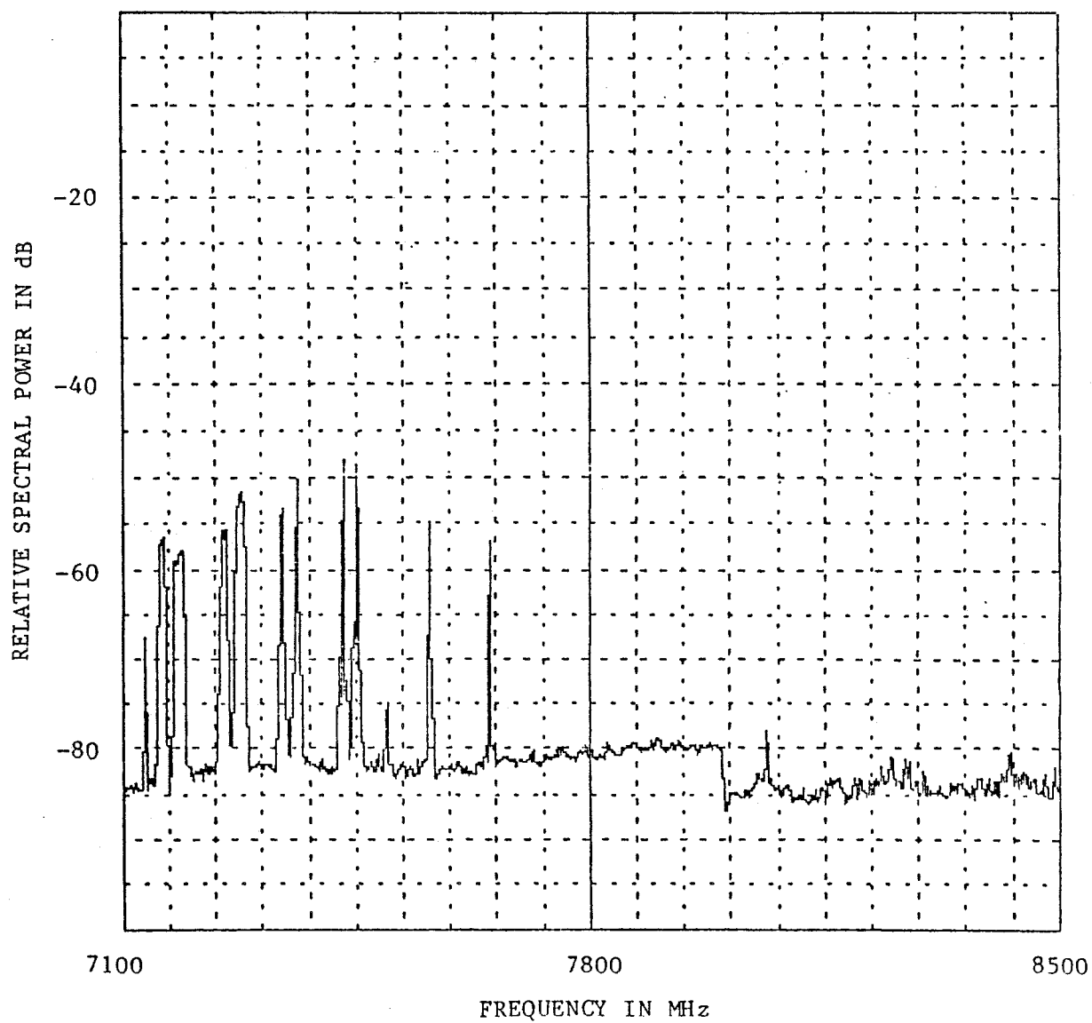
Figure A-63. Band Scan of the Madrona - Auburn Antenna.
