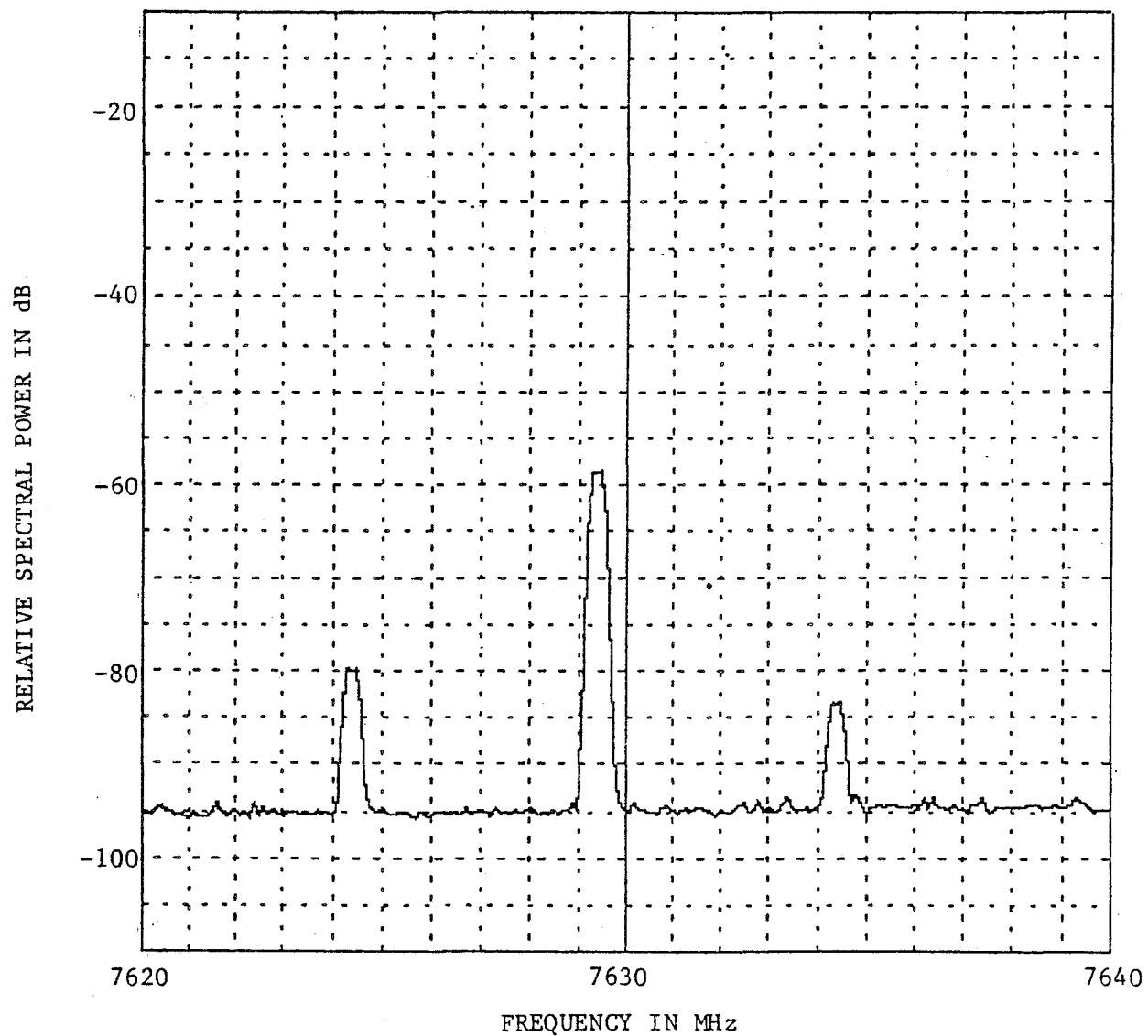
Figure A-60. Emission Spectrum of a Collins 552A-5 ( f_o = 7630 MHz, Radiated).
