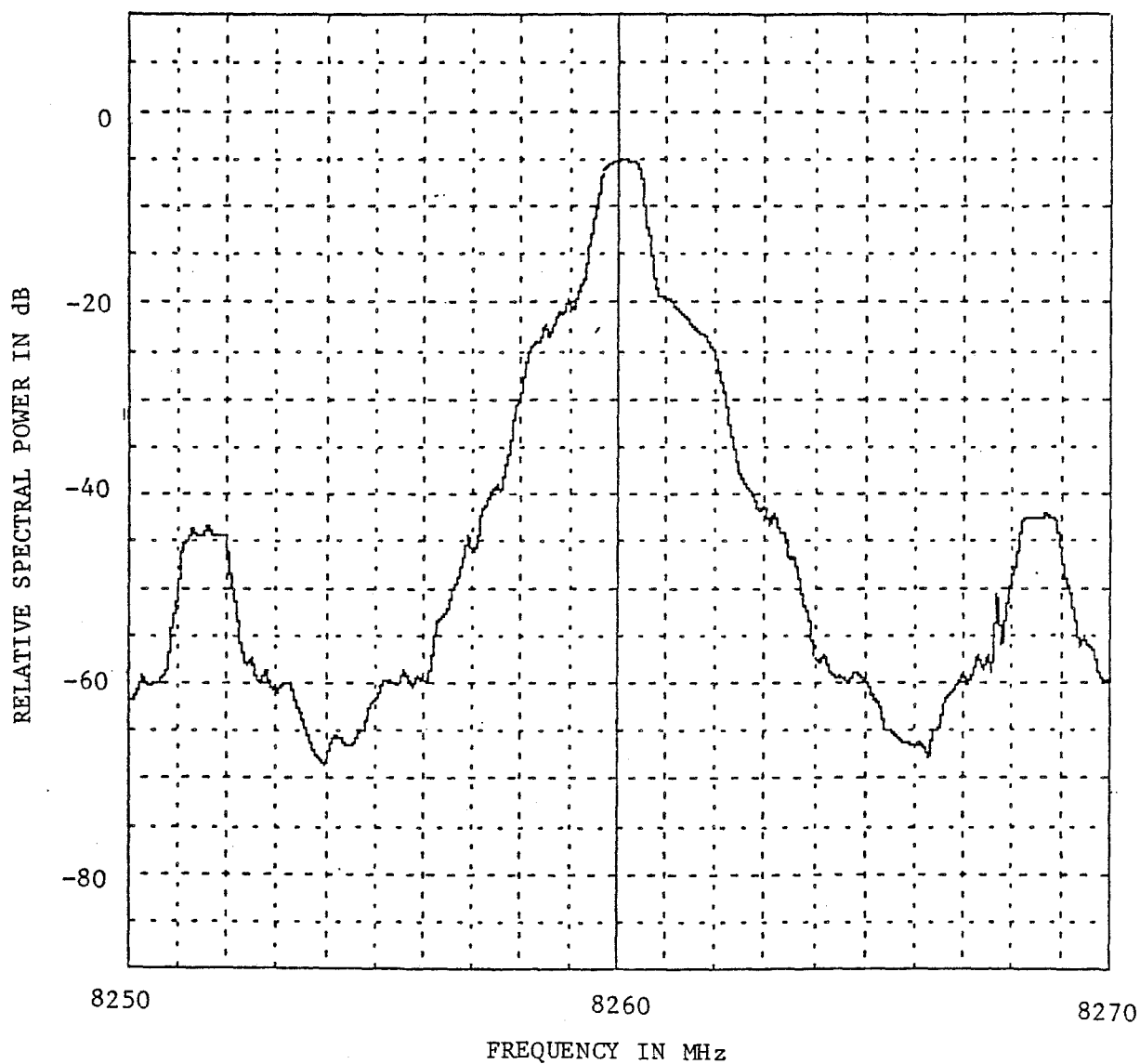
Figure A-30. Emission Spectrum of a General Electric TRS696C ( f_o = 8260 MHz, Hard-lined).
