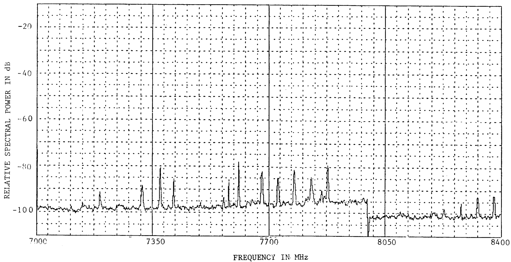
Figure A-1. Band Scan at Blyn Mountain - 7000 to 8400 kHz.
