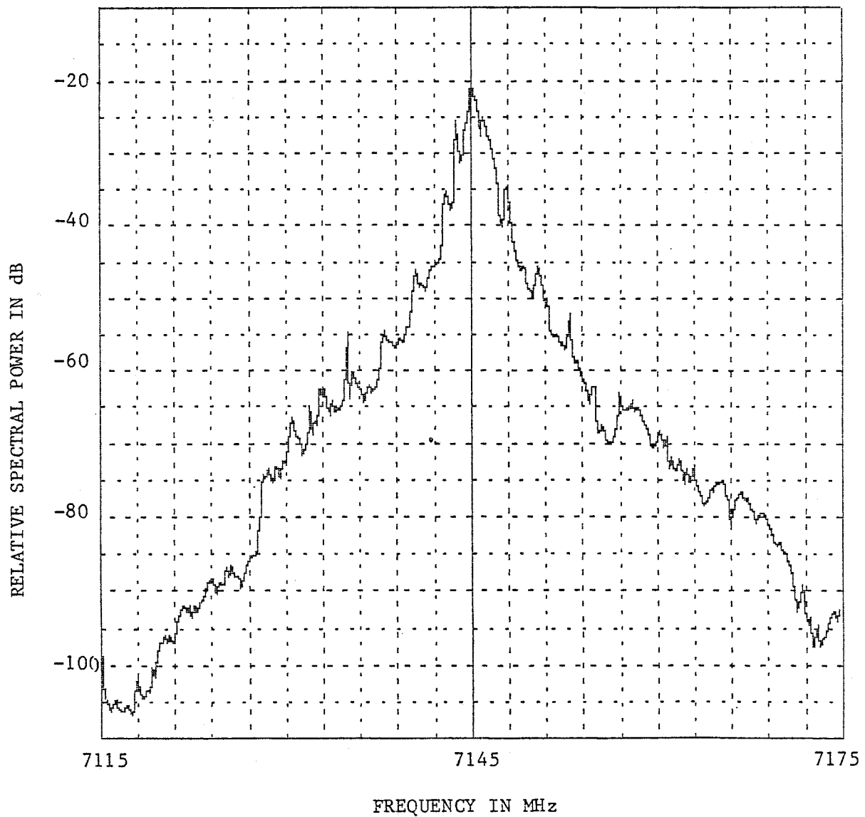
Figure A-14. Emission Spectrum of a Farinon Electric FV8F ( f_o = 7145 MHz Hard-lined).
