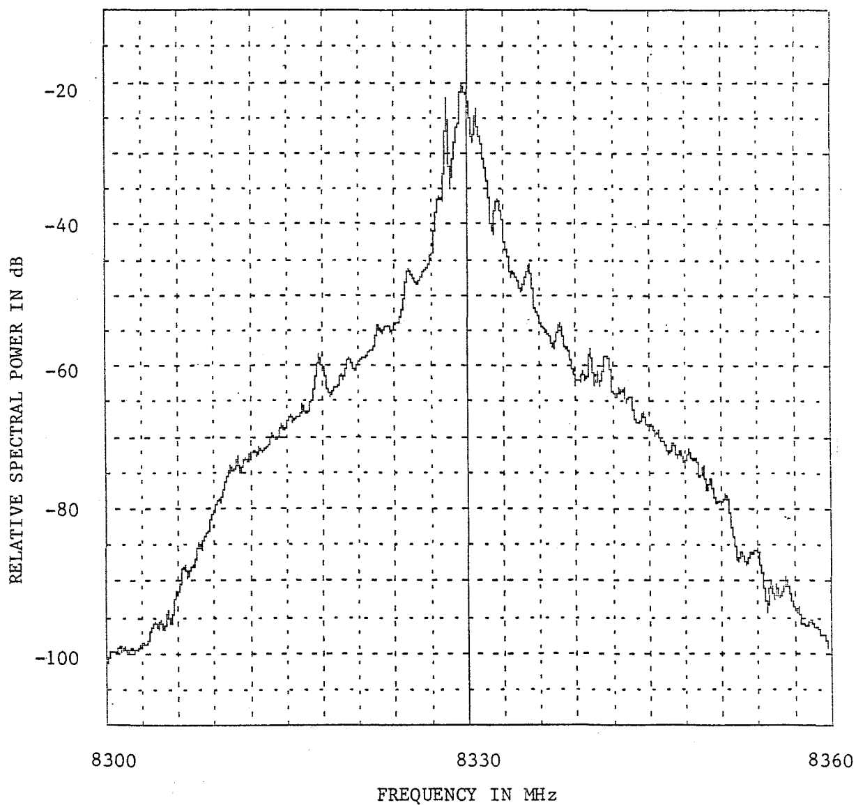
Figure A-19. Emission Spectrum of a Farinon Electric FV8F ( f_o = 8330 MHz, Hard-lined).
