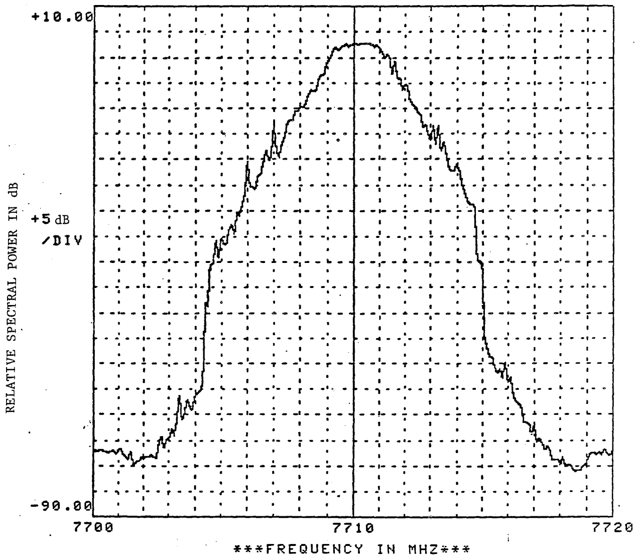
Figure 15. Transmitter Emission Spectrum of a Collins MW508C.
